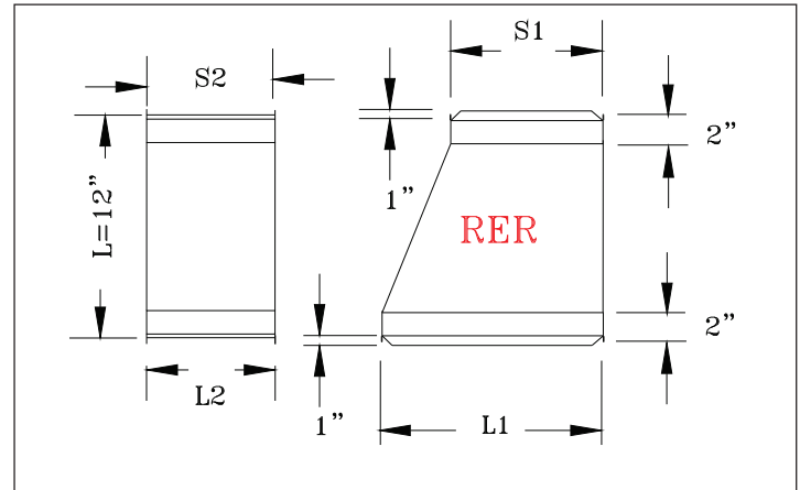
Rectangular Eccentric Reducer.
