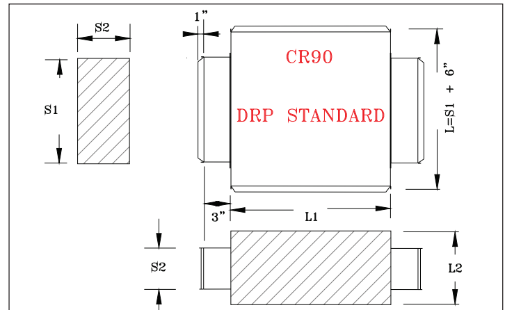
90° Rectangular Cross.
