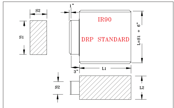
90° Rectangular Lateral.
