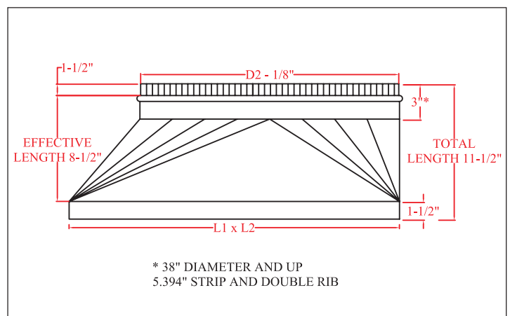
Eccentric Reducer
