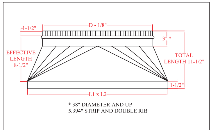
Concentric Reducer
