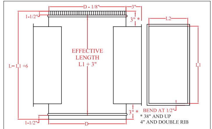
Squared Cross
