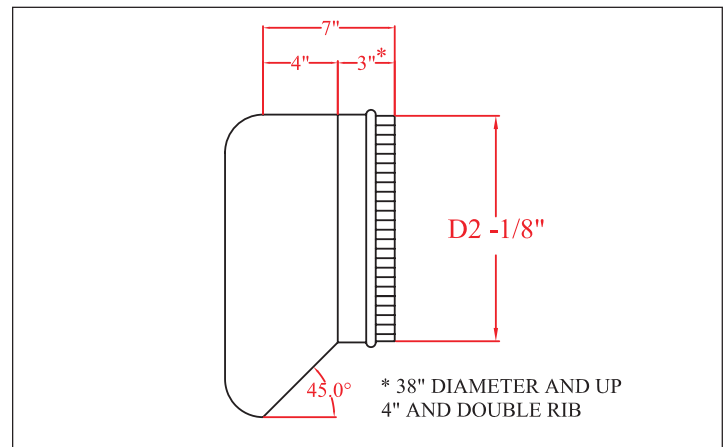
Round Reducer cap
