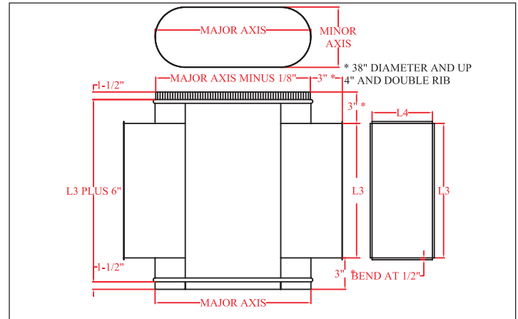
Oval 90° Cross to Rectangular.
