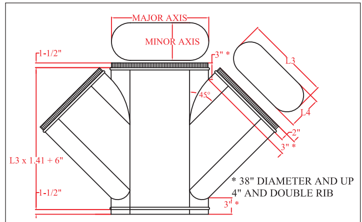
Oval 45° Horizontal Cross
