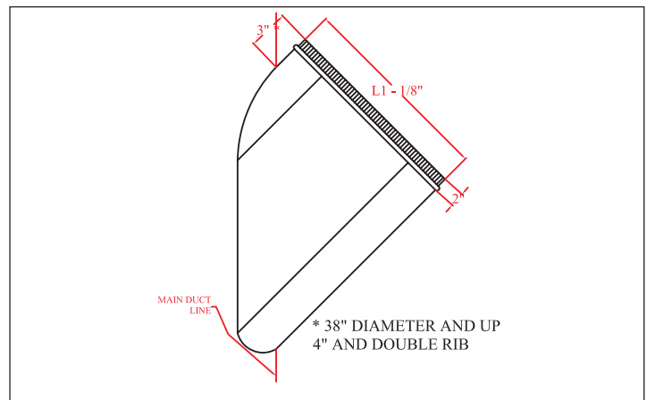
Oval 45° Horizontal Tap
