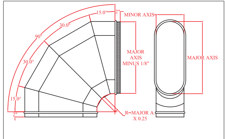
Oval 90° Horizontal Elbow
