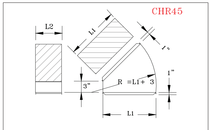
Rectangular 45° Horizontal Elbow.
