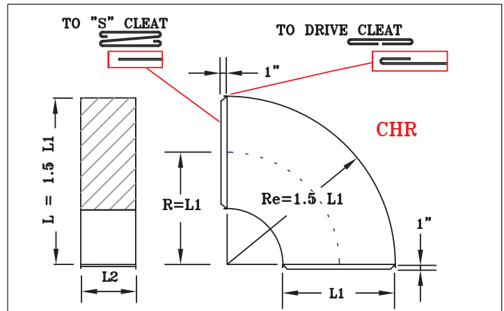
Rectangular 90° Horizontal Elbow.
