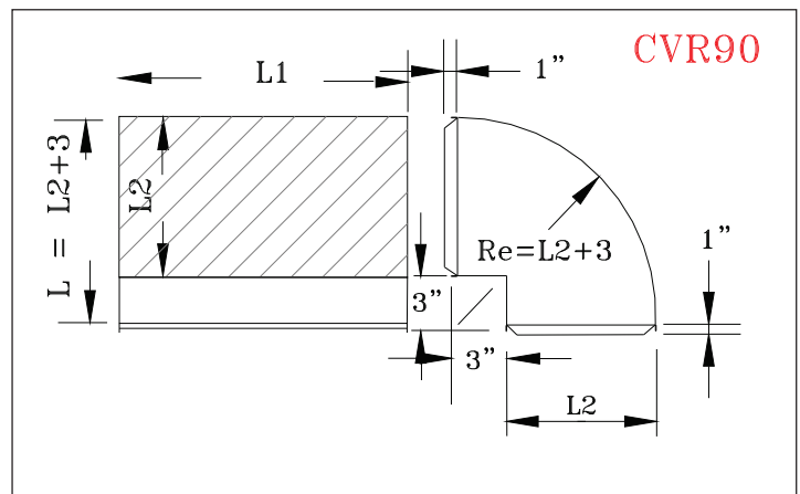
Rectangular 90° Vertical Elbow.
